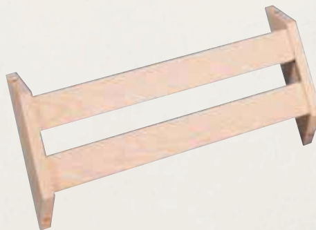
4224 Hymn Book Rack unfinished 4225 Hymn Book Rack finished Inside dimensions: 18"w x 2-1/4"d Outside dimensions: 20"w x 3"d, 9"h
